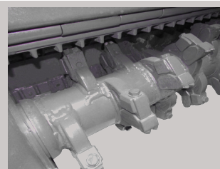
Wrap around rotor blade holder & tungsten carbide tips
